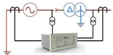
Figure 2 P346 for synchronization check
