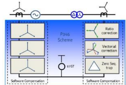
Figure 1 P346 for transformer differential protection
