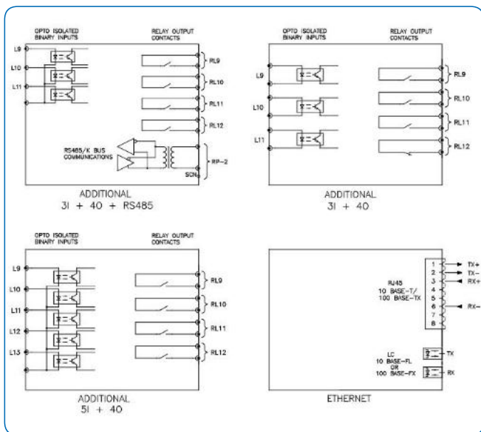
Example hardware options available in case size 30TE
