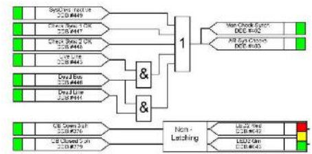
Programmable Scheme Logic
